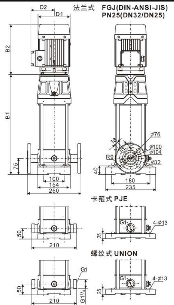
安装图/Installation sketch
