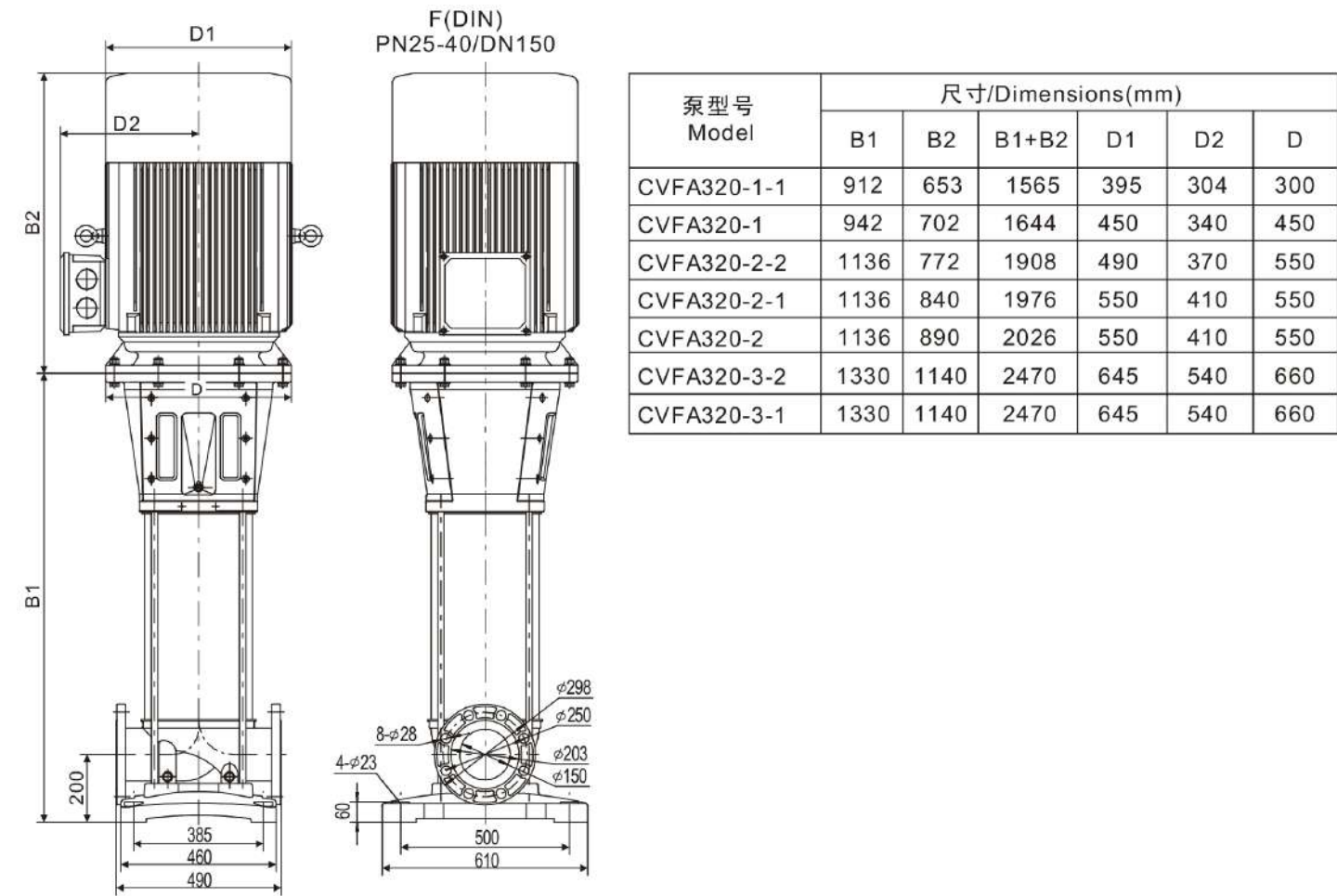
安装图/Installation sketch
