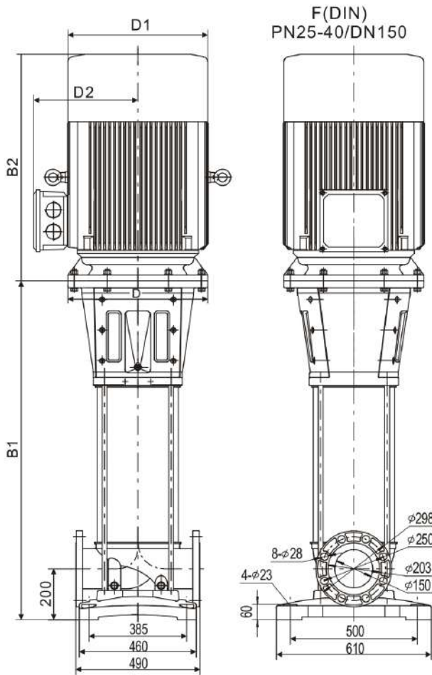
安装图/Installation sketch
